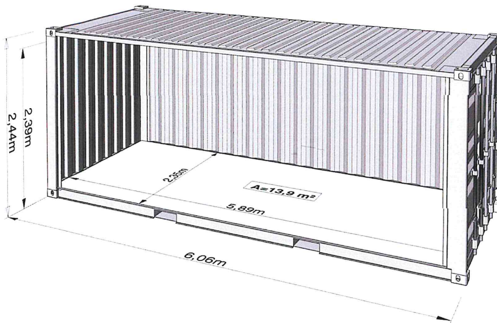
FIGURE 2 – EXAMPLE OF THE STORAGE CONTAINER
